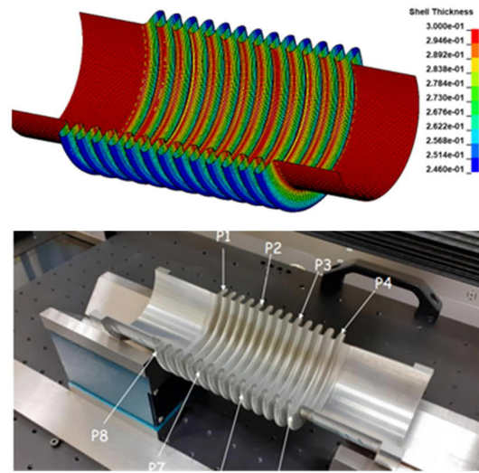
Figure 3. Top: simulation of the hot forming for the ATLAS bellows. Bottom: experimental test [6].
