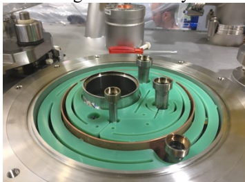
Figure 10: Jumper centering part on cryomodule.
