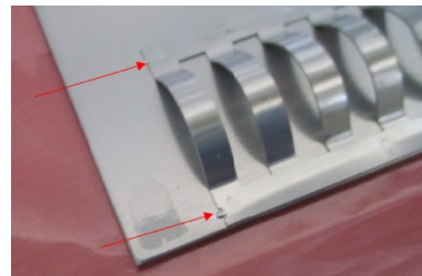
Figure 9: Flexible contact of first DQW prototype welded at both extremities.
