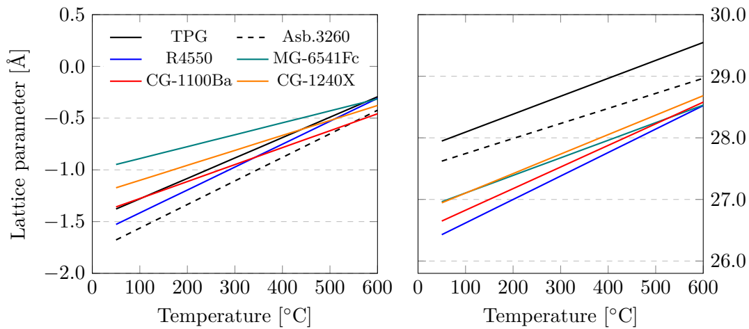
Figure 6.11: Result of the secant CTE 20-T °C of graphite ( \times 10^{-6} m^{-1} K^{-1} ): a (left), c (right).
