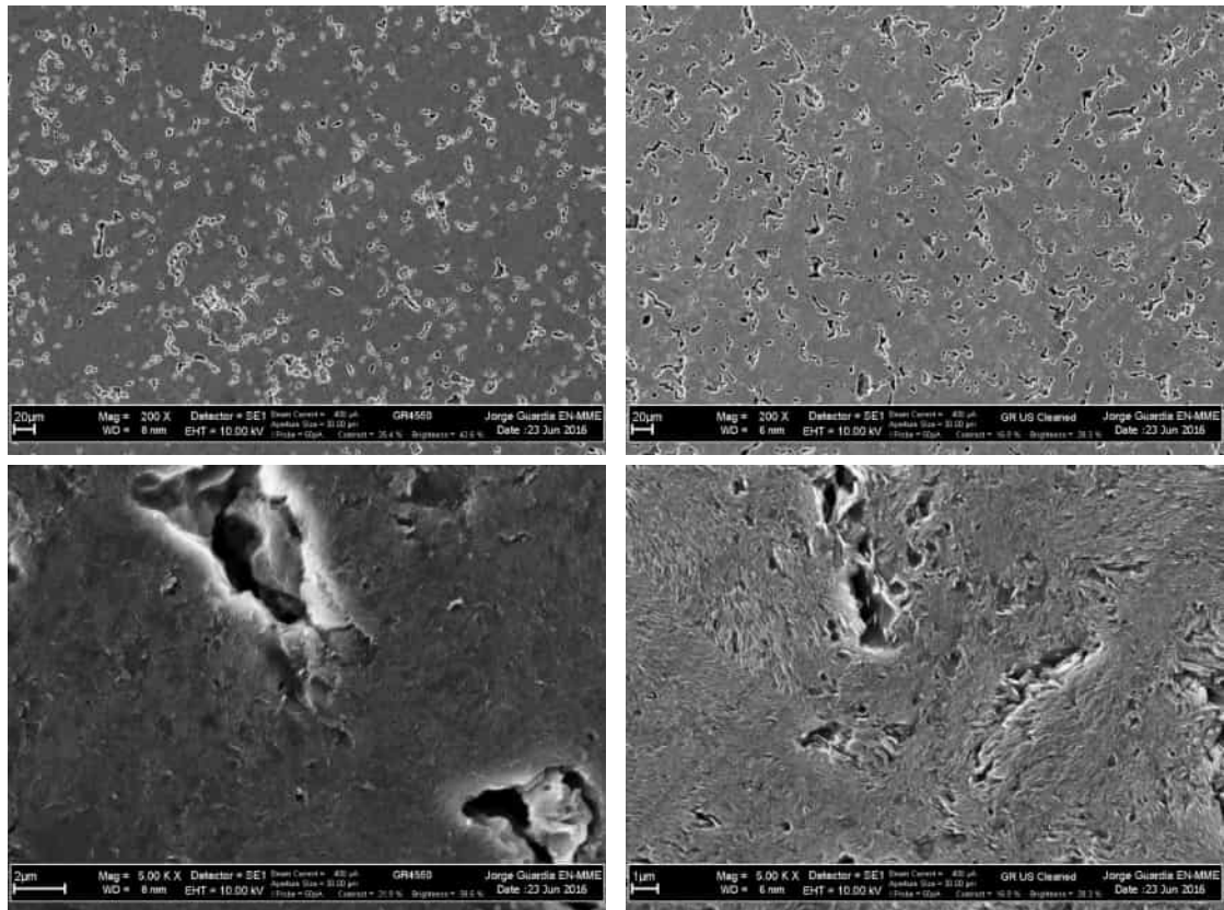
Figure 6.19: Graphite R4550 polished surface by SEM, before (left) and after (right) sonication.
