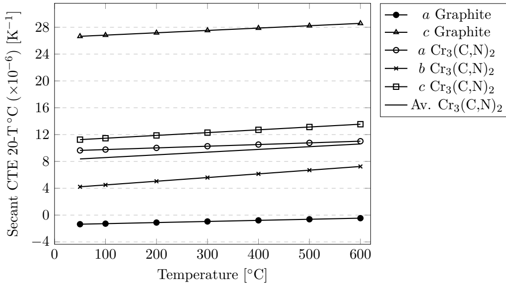
Figure 5.47: Secant CTE 20-T °C of graphite and \text{Cr}_3(\text{C,N})_2 in CG-1100Ba (from XRD).
