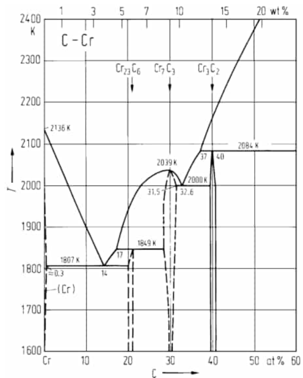
Figure 2.17: Phase diagram of the chromium-carbon system [103]. There is one peritectic reaction at \text{Cr}_{60}\text{C}_{40} ( 1811^\circ\text{C} ), in equilibrium with solid C. The peritectic liquid (100% liquid) has \text{Cr}_{63}\text{C}_{37} ; during cool down, it forms \text{Cr}_3\text{C}_2 and the liquid moves to the eutectic reaction \text{L}(\text{Cr}_{67.4}\text{C}_{32.6}) \leftrightarrow \text{Cr}_7\text{C}_3 + \text{Cr}_3\text{C}_2 , which is not in equilibrium with solid C. However, with excess carbon, only \text{Cr}_3\text{C}_2 is formed from the LP, solidifying completely at 1811^\circ\text{C} .
