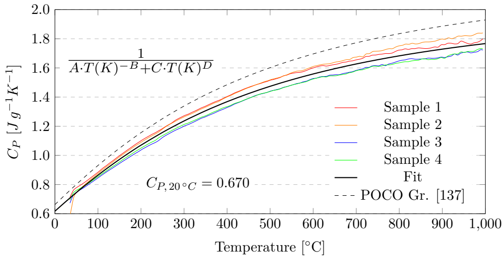
Figure 5.52: Specific heat of MG-1100Ba. Fitting equation constants: A = 11.77 , B = 1.644 , C = 4.047\text{E-}4 and D = 0.02191 .
