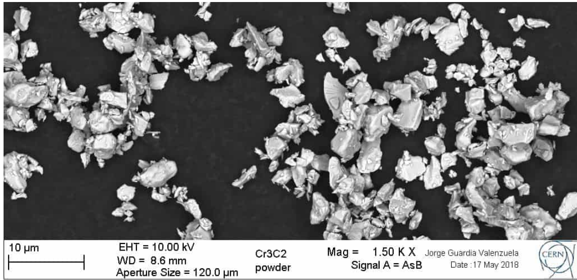
Figure 4.28: Typical morphology of the \text{Cr}_3\text{C}_2 powder (SEM). Backscattered electron detector.
