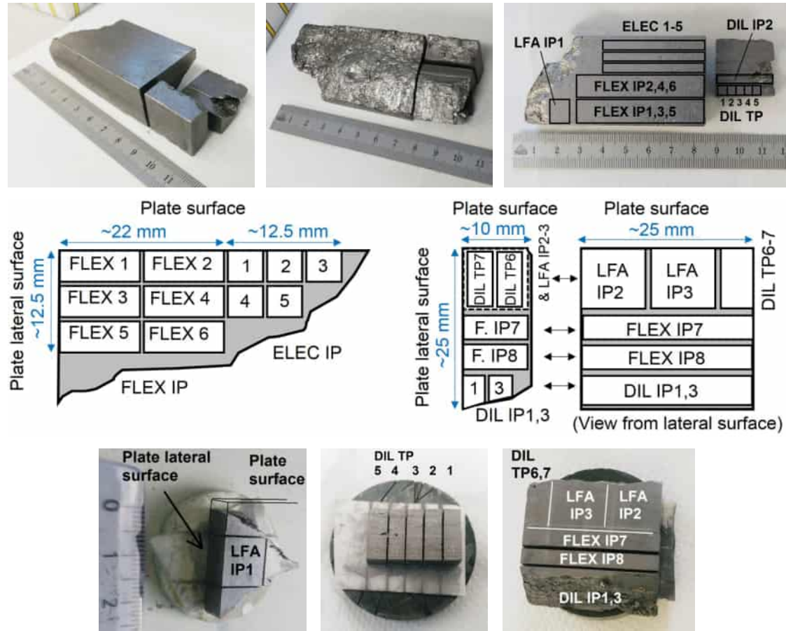
Figure 5.84: Specimens for characterisation obtained from CG-1240X plate.
