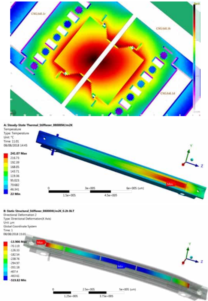
Figure 1.20: Example of collimator design validation iteration.
