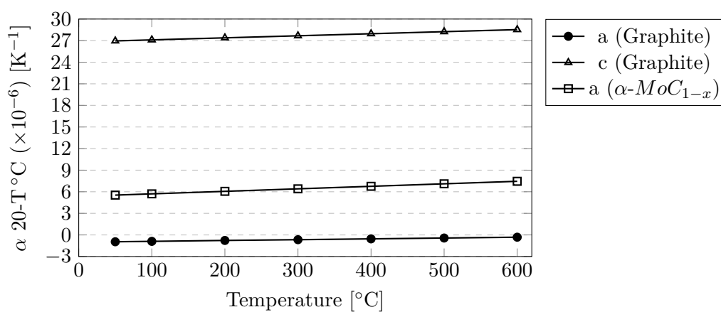
Figure 5.32: Secant CTE 20-T^{\circ}\text{C} of graphite and \alpha\text{-MoC}_{1-x} in MG-6541Fc (from XRD).
