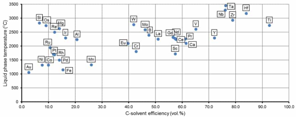
Figure 2.18: Carbon solvent efficiency versus (minimum) liquid phase temperature.
