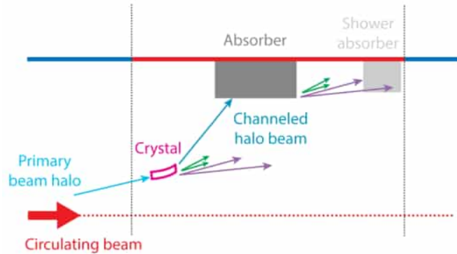
Figure C.3: Schematic of crystal collimation [16].
