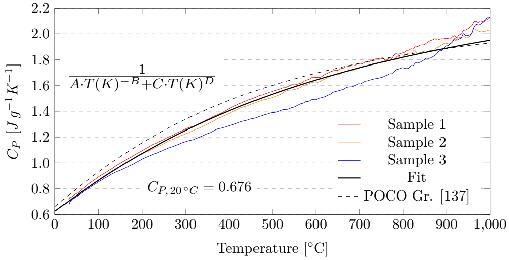
Figure 5.35: Specific heat of MG-6541Fc. Fitting equation constants: A = 3.860 , B = 1.437 , C = 3.786\text{E-}4 and D = 3.779\text{E-}4 .
