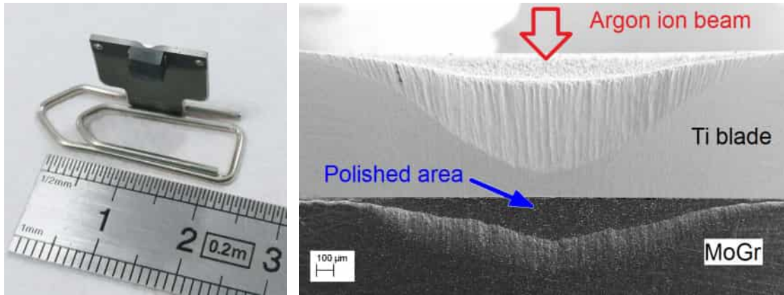
Figure 3.27: (Left) MoGr sample ( \sim 4 \times 4 \times 2 mm) mounted on the blade. (Right) SEM image of the finished ion-polishing process.
