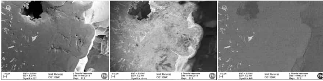
Figure 6.35: SEM observations of the LP spill from CG-1100A0 cycle. The images correspond to the polished surface, but the external droplet surface is also visible at the bottom right area of the three images. From left to right: SE, SE and BE detector images. Note how the BE image does not show carbide content at the droplet external surface.
