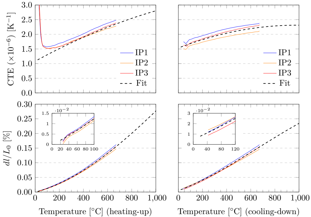
Figure 5.97: CTE CG-1240X IP. All specimens with length \approx 25\text{ mm} . Fitting polynomials are all 3 th degree.
