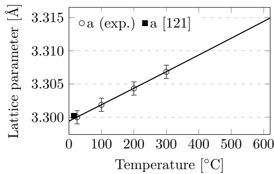
Figure 3.24: Niobium lattice parameter versus temperature, matching a_{15^\circ\text{C}} = 3.3002 \text{ Å} [121].
