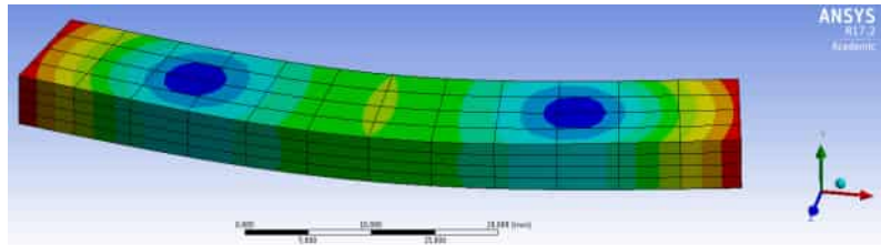
Figure E.11: First flexural mode in a non desired orientation (mode 8, 12963 Hz).
