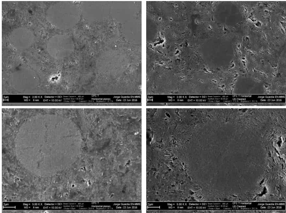
Figure 6.18: CFC AC150K TP polished surface by SEM, before (left) and after (right) sonication.
