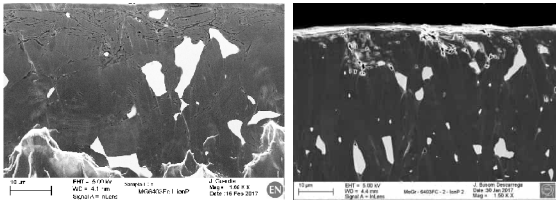
Figure 6.13: Low magnification SEM observations of ion-polished MG-6403Fc. (Left) case B and (right) case A from Figure 6.12.
