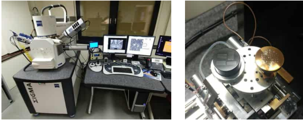
Figure 3.26: (Left) SEM Zeiss Sigma. (Right) MoGr specimens mounted in a black resin cylinder on the SEM sample holder, together with a piece containing several reference samples for EDS analysis.
