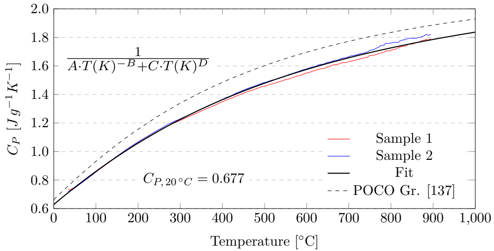
Figure 5.62: Specific heat of MG-1100A0. Fitting equation constants: A = 4.284 , B = 1.462 , C = 4.098\text{E-}4 and D = 3.748\text{E-}3 .
