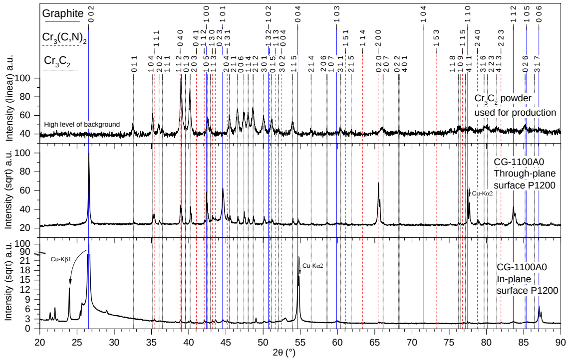
Figure 5.59: CG-1100A0 IP and TP XRD patterns.
