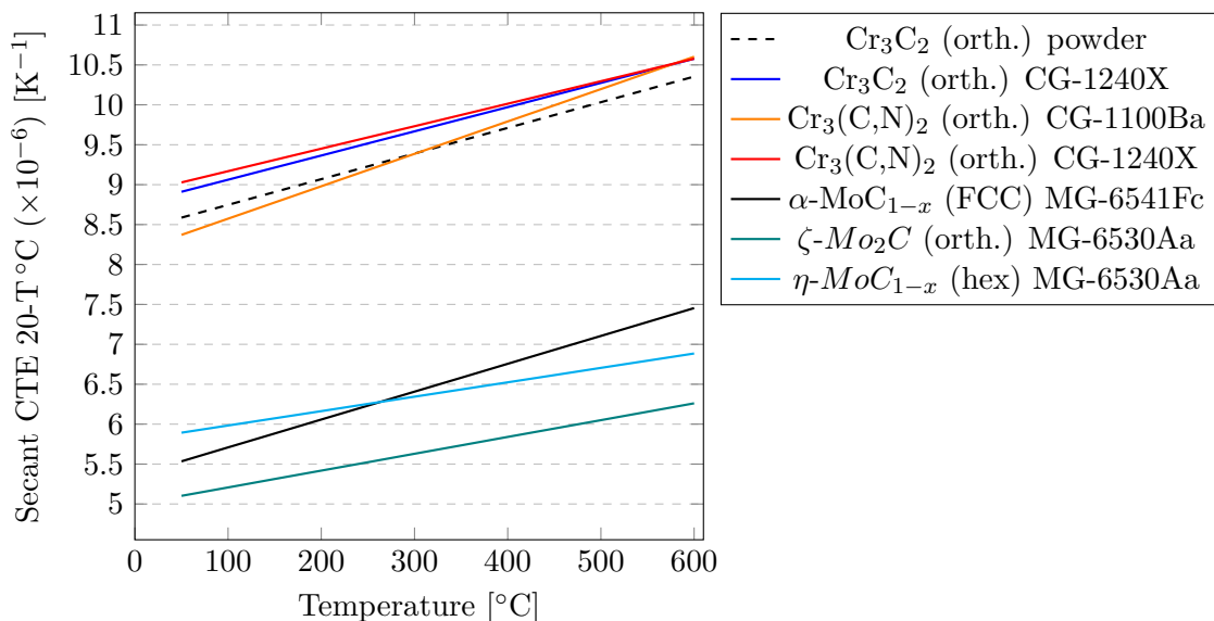
Figure 6.7: Secant CTE 20-T °C of chromium and molybdenum carbides, directional average.
