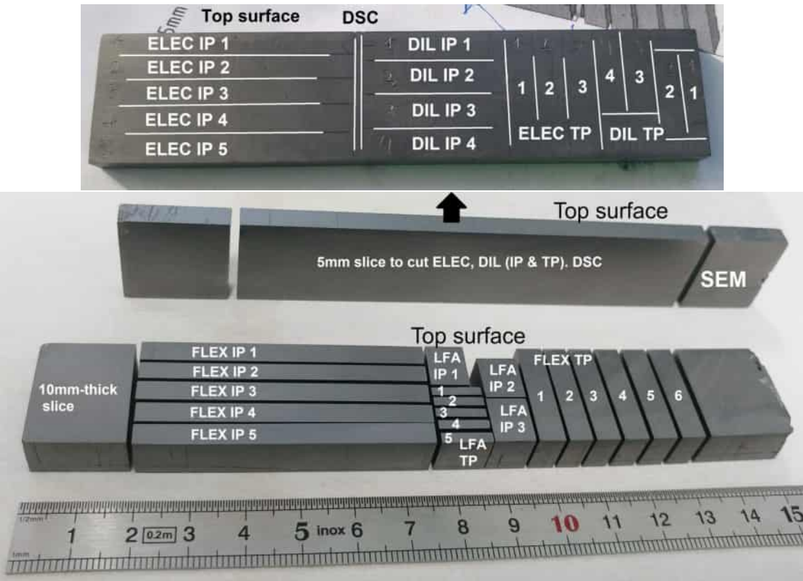
Figure 5.68: Plate location of all CG-1100B0 specimens, cut with diamond wire saw.
