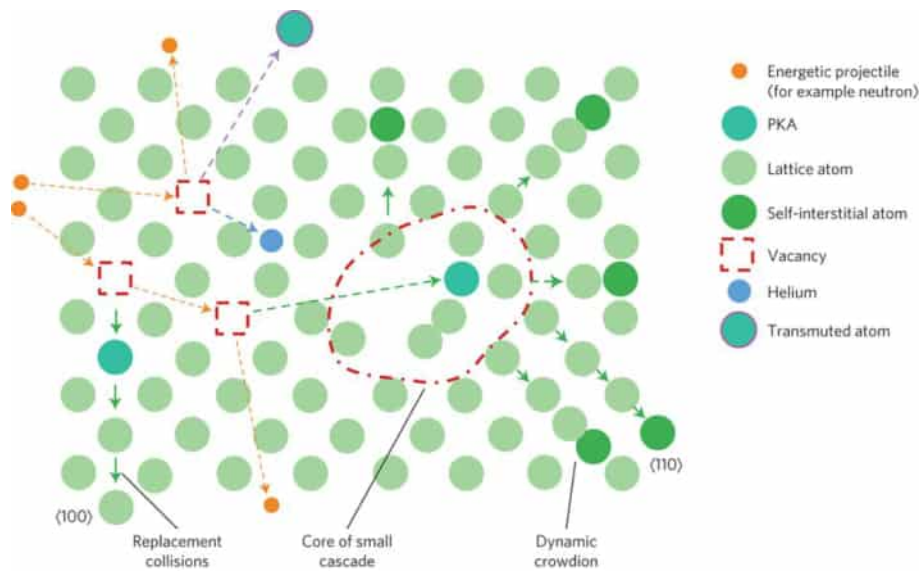
Figure D.2: Schematic of radiation damage, showing both elastic and inelastic (transmutation) interactions [166]. Reprinted by permission from Springer Nature.
