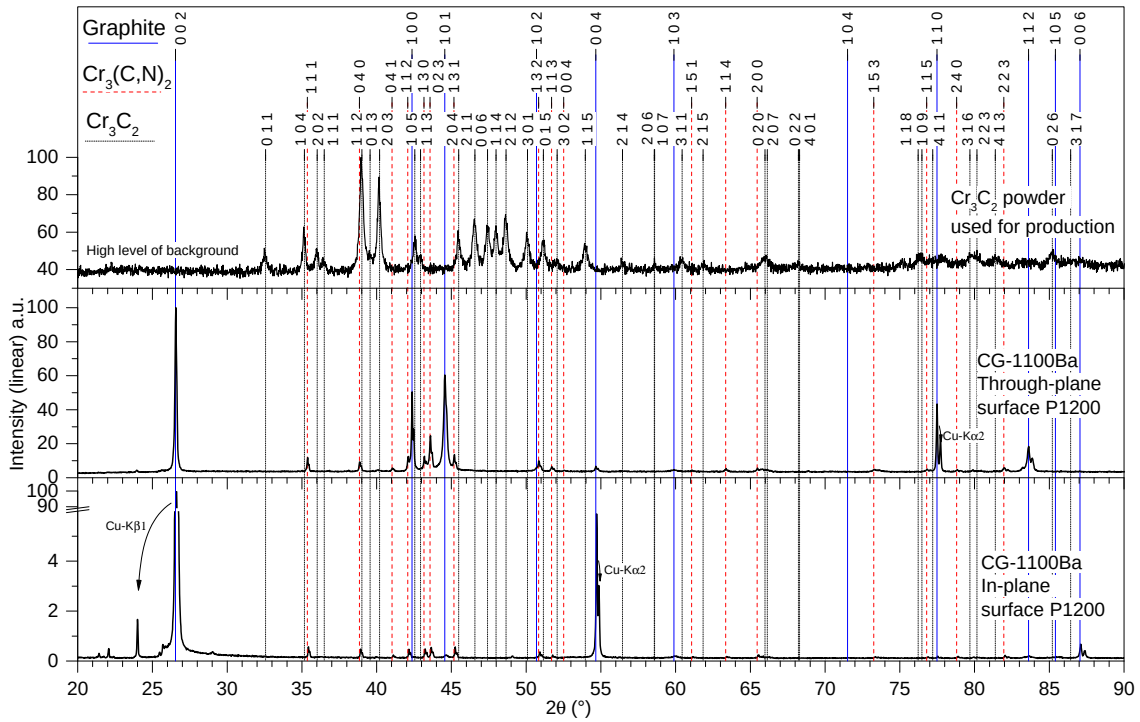
Figure 5.42: CG-1100Ba IP and TP XRD patterns.
