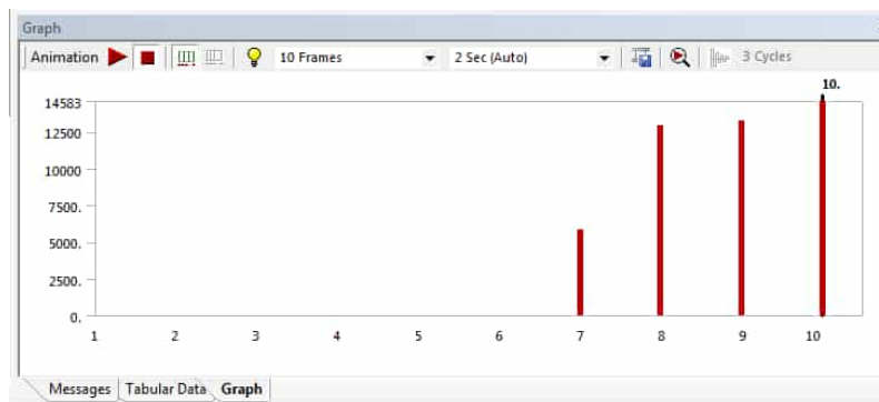
Figure E.9: Plot of the frequencies of the first 10 modes of an IP free-standing specimen. The first 6 modes with F \approx 0 \text{ Hz} are the degrees of freedom.
