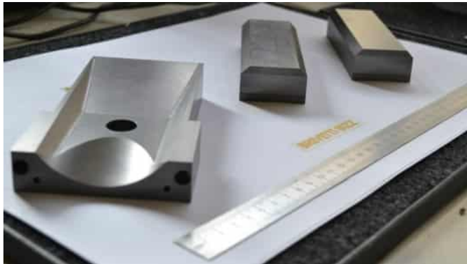
(a) MG-6530Aa machined blocks for full-size collimator test. External dimensions of the parts shown are 150 \times 100 \times 25 \text{ mm} or 125 \times 45 \times 25 \text{ mm}
