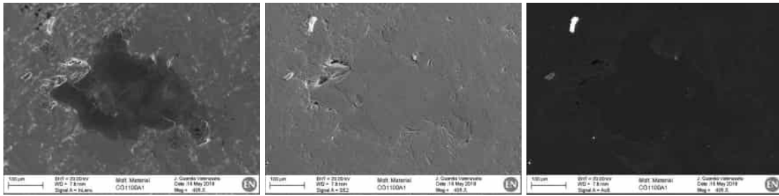
Figure 6.31: SEM observations of a graphite flake in the LP spill from CG-1100A0 cycle oriented parallel to the surface. From left to right: SE, SE and BE detector images.
