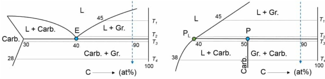
Figure 2.13: (Left) Eutectic system. (Right) Peritectic system.
