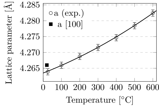
Figure 5.31: Lattice parameters versus temperature of \alpha\text{-MoC}_{1-x} in MG-6541Fc.
