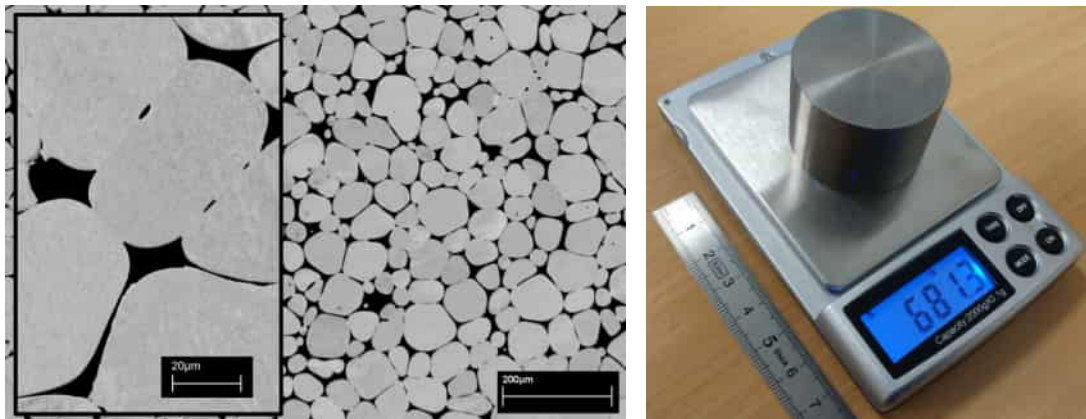
Figure 1.24: (Left) Microstructure of INERMET®180 by SEM backscattered electron detector: bright grains are tungsten and dark areas are the Cu-Ni matrix [29]. (Right) Weight of a cylinder of INERMET®180 alloy with size \varnothing 40 \times 30\text{ mm} : 681 g.
