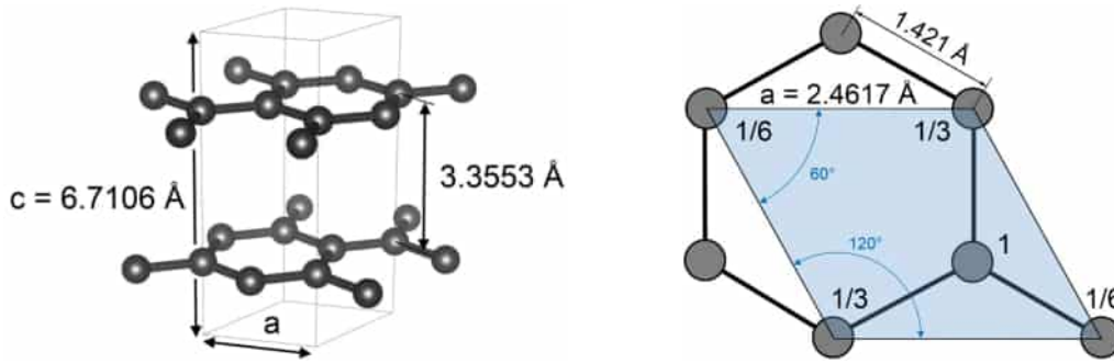
Figure 3.12: (Left) Unit cell of graphite crystal structure. (Right) Number of carbon atoms at each of the two basal layers in the unit cell.
