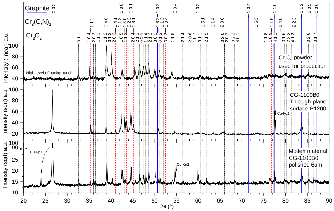
Figure 5.72: CG-1100B0 TP and molten material XRD patterns.
