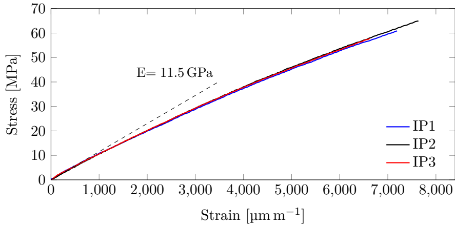
Figure 5.25: Bending test of graphite R4550.
