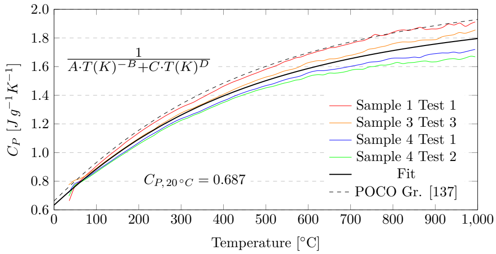
Figure 5.77: Specific heat of CG-1100B0. Fitting equation constants: A = 11.42 , B = 1.644 , C = 3.993\text{E-}4 and D = 0.02191 .
