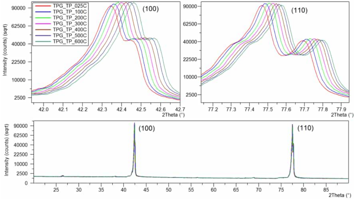
Figure 5.6: TPG TP experimental XRD patterns.
