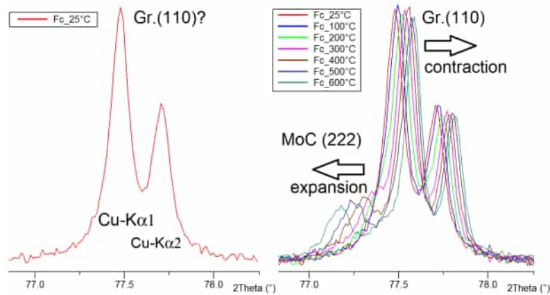
Figure 5.29: Graphite (110) and \alpha - \text{MoC}_{1-x} (220) overlapped peaks shifting in opposite directions.
