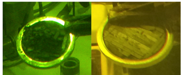
Figure 1: Observed structural degradation in MG-1110E samples after irradiation with 1.1 \times 10^{21} p/cm 2 by 160 MeV protons (left) and exposure to 2.8 \times 10^{18} p/cm 2 at 160 MeV followed by fast neutron fluence of 3.2 \times 10^{18} n/cm 2 (right).
